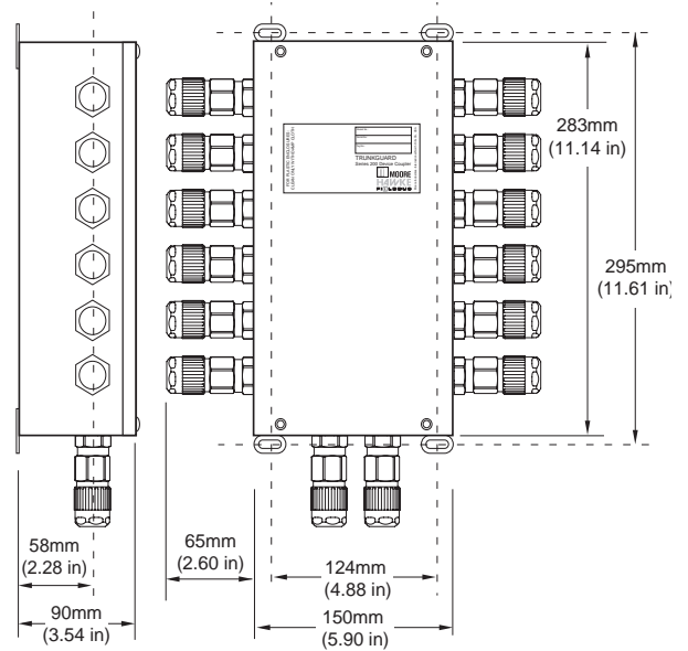
Figure 7. Electro-Polished Stainless Steel 316 Enclosure Installation Dimensions for 8-Spur (TG228) and 10-Spur (TG22X) Models.
