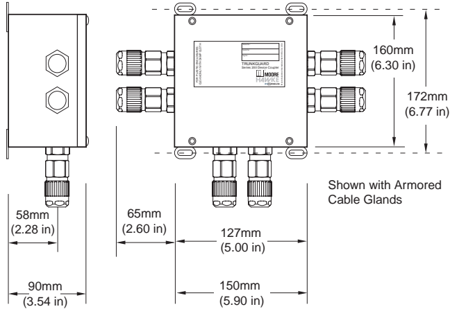
Figure 6. Electro-Polished Stainless Steel 316 Enclosure Installation Dimensions for 4-Spur (TG224) Models.
